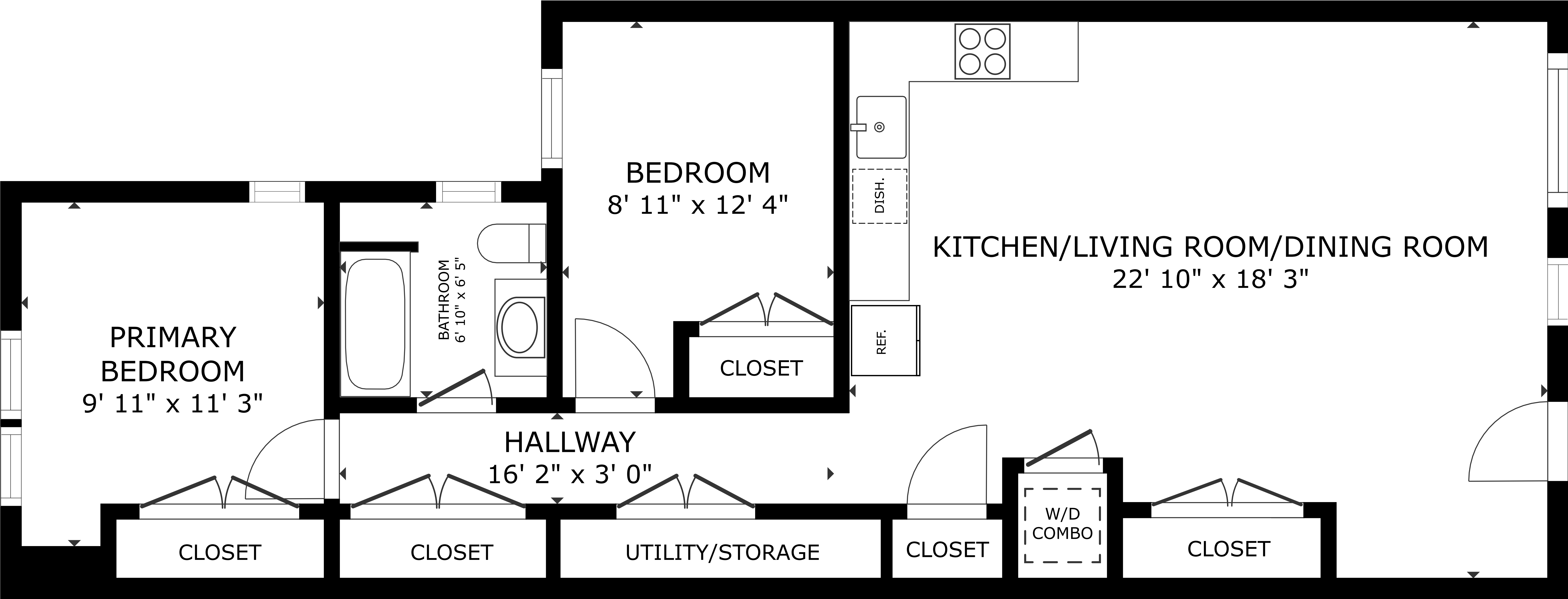
FLOOR PLAN
